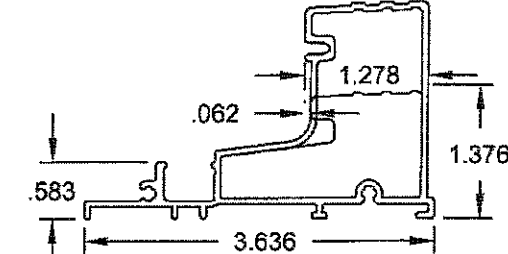
⑩ #8058A 6063-T6 OUT-SWING LOW SILL
