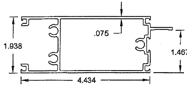
⑤⑤ #8014A 6063-T5 TOP RAIL, LAG BOLT DESIGN
