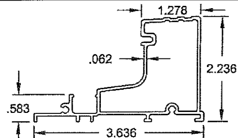
② #8003C 6063-T6 OUT-SWING SILL
