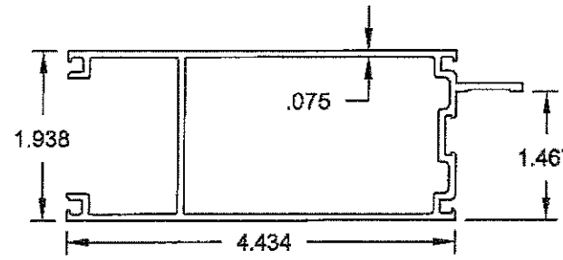
㉑ #8014 6063-T5 TOP RAIL
