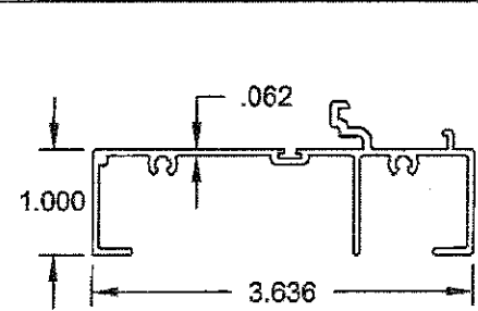
① #8006 6063-T6 FRAME, HEAD, JAMB AND SIDELITE SILL
