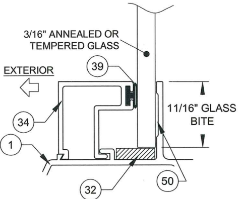
GLASS TYPES 3 & 4
