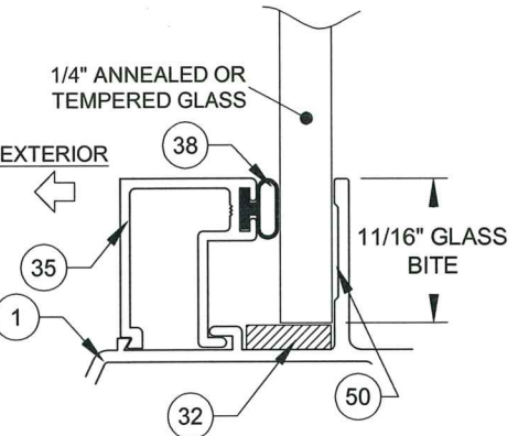
GLASS TYPES 5 & 6
