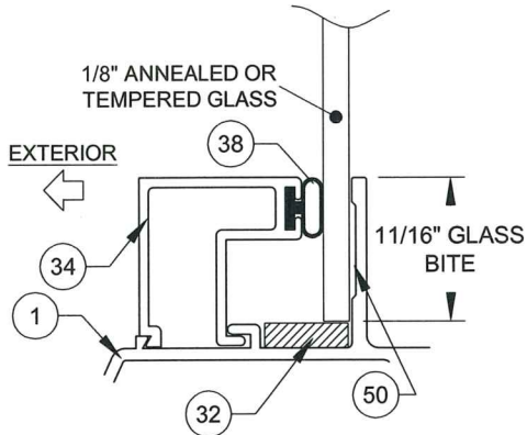
GLASS TYPES 1 & 2
