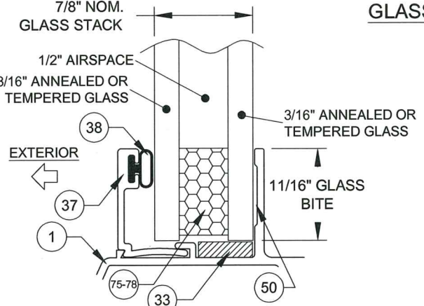
GLASS TYPES 9 & 10
